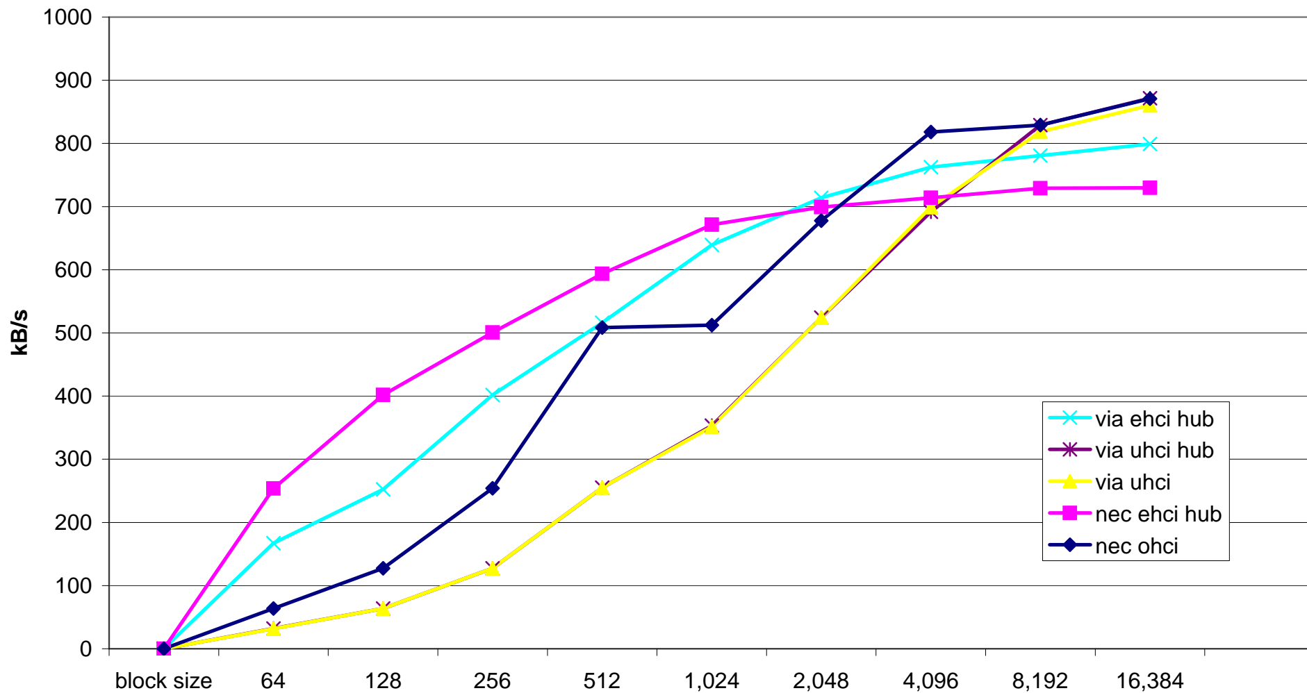
LPCUSB throughput of 'custom' application
